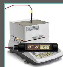
external calibration thermometer
